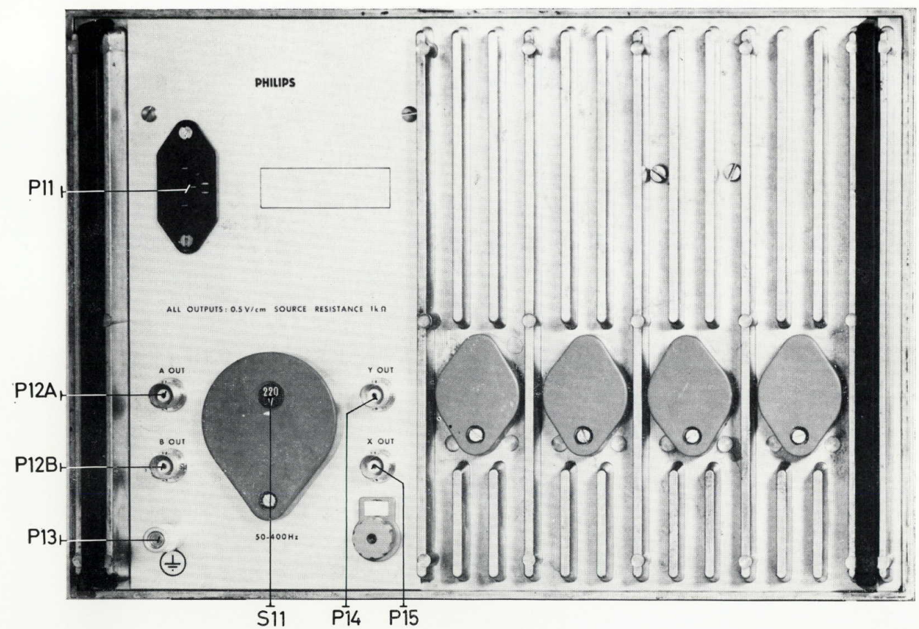
Fig. VI-5 Controls and sockets on the rear of the instrument
