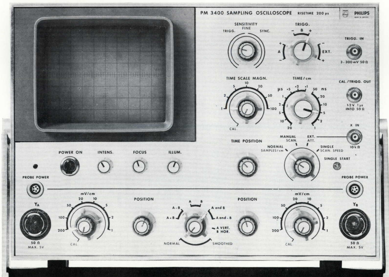
Fig. V-1 Front view
