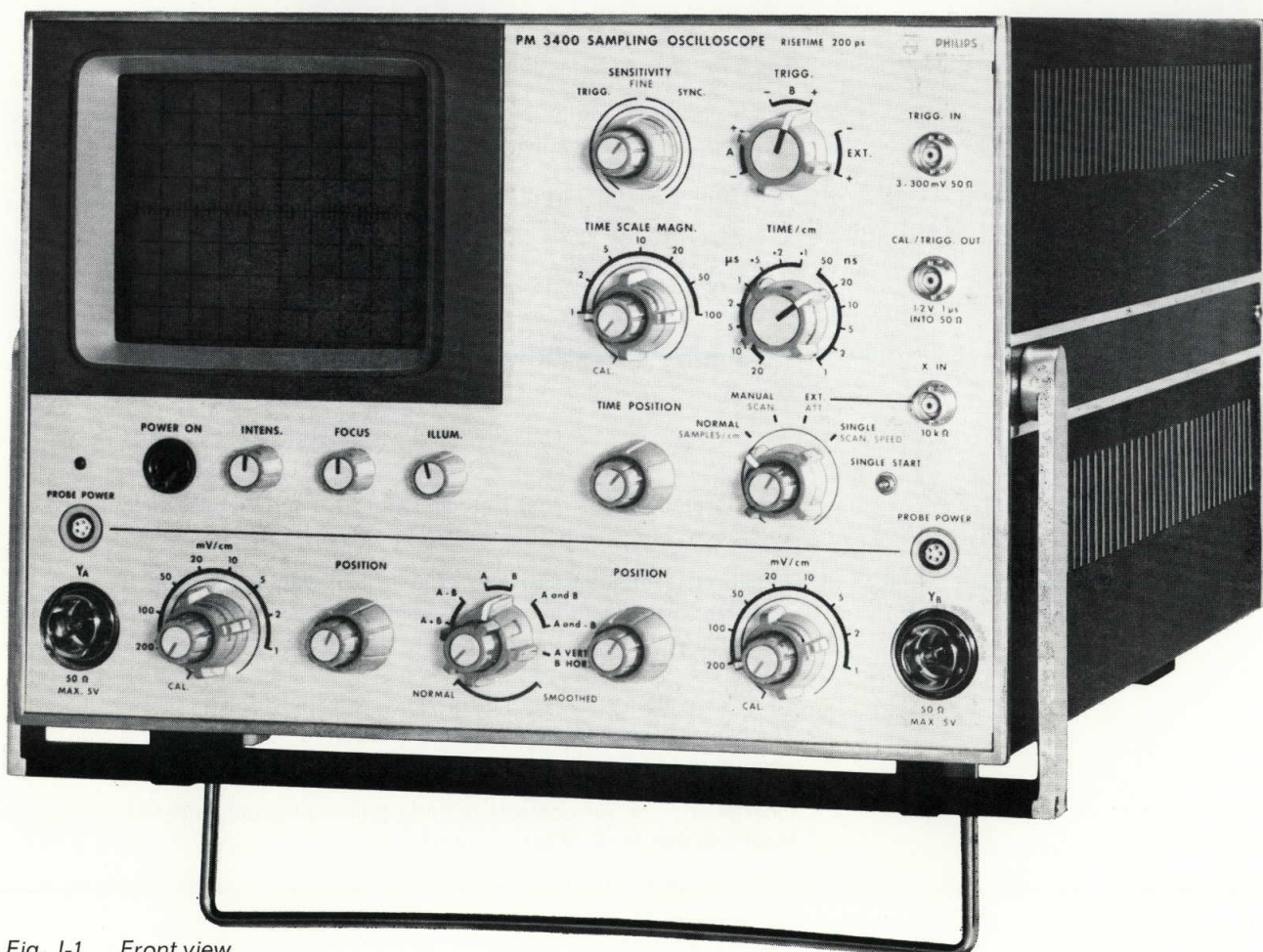
Fig. I-1 Front view
