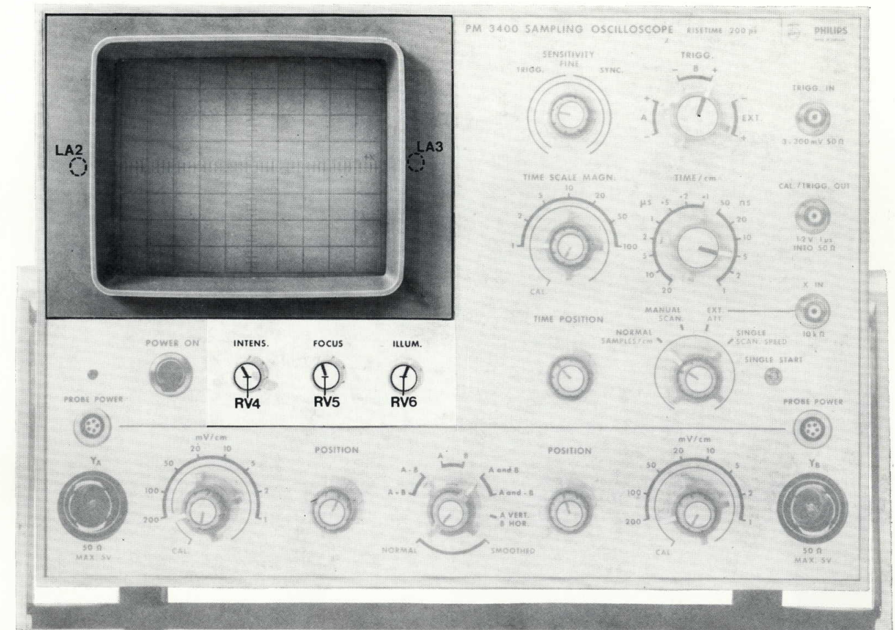
Fig. VI-3 Controls and sockets DISPLAY
