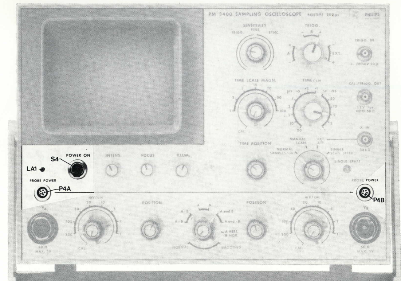
Fig. VI-4 Controls and sockets POWER SUPPLY
