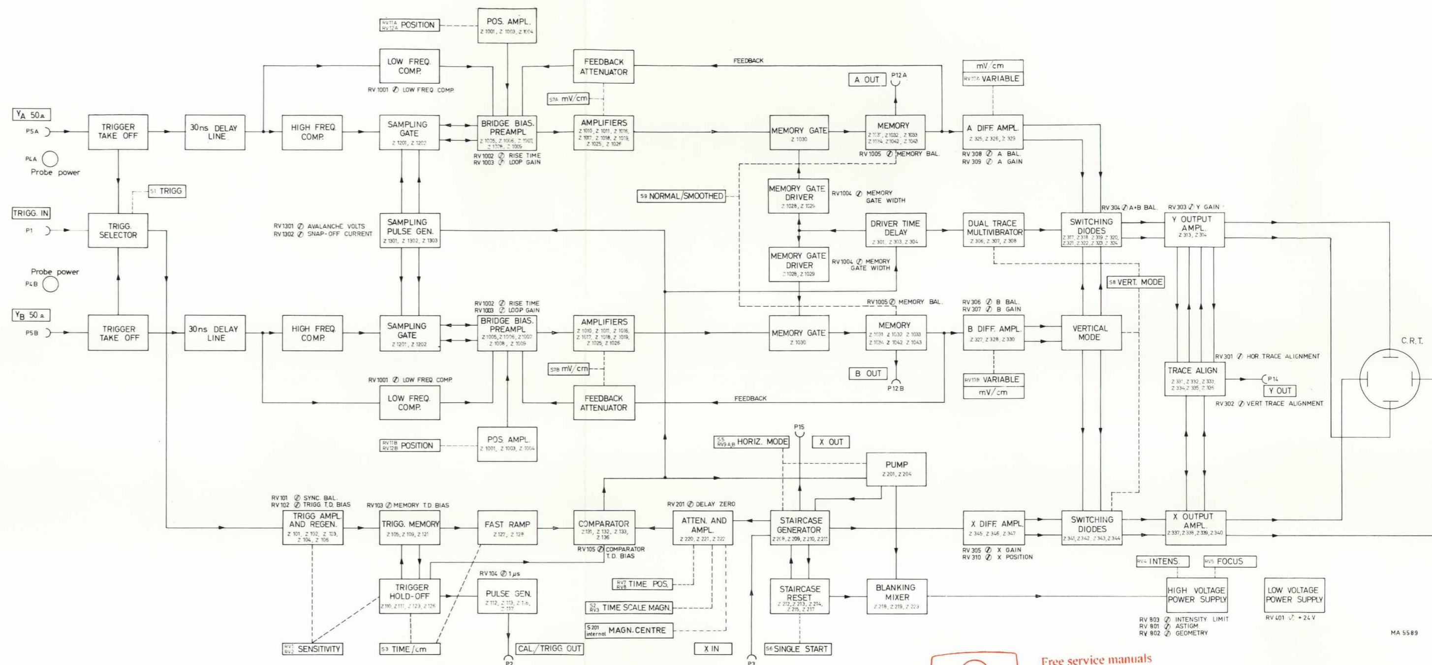
Fig. IV-1 Block diagram
